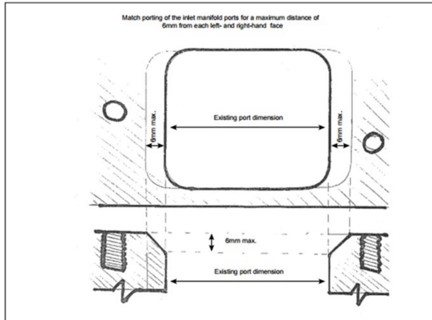
Match porting of inlet manifold
